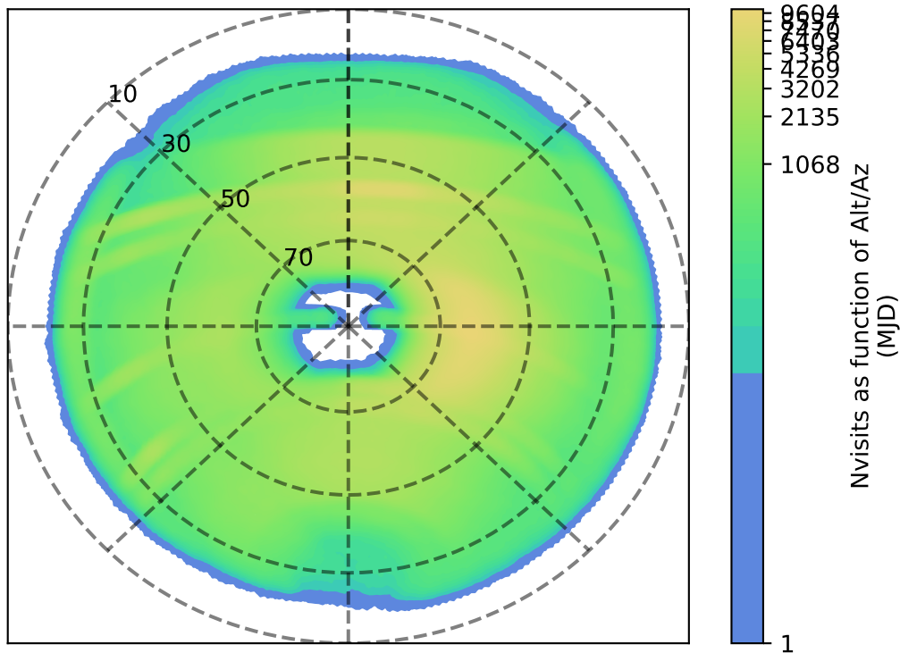
weather_cloudso8v3.4_10yrs : Nvisits as function of Alt/Az
