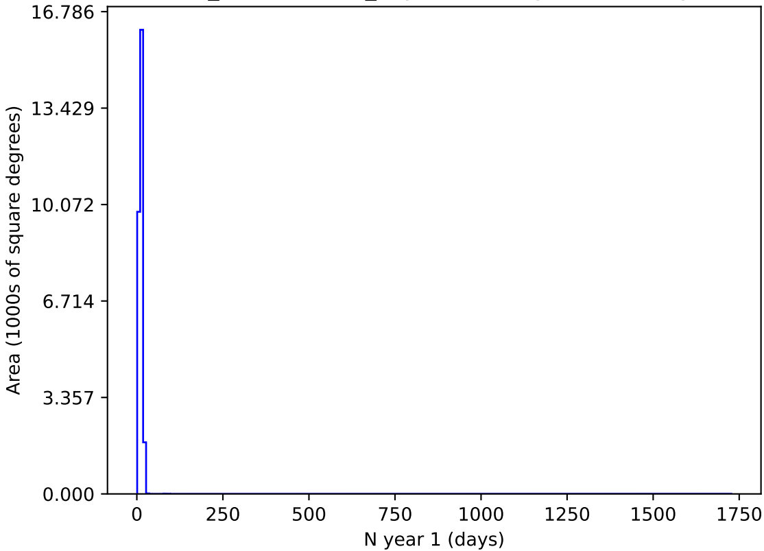
weather_cloudso8v3.4_10yrs z and night < 365: N year 1
