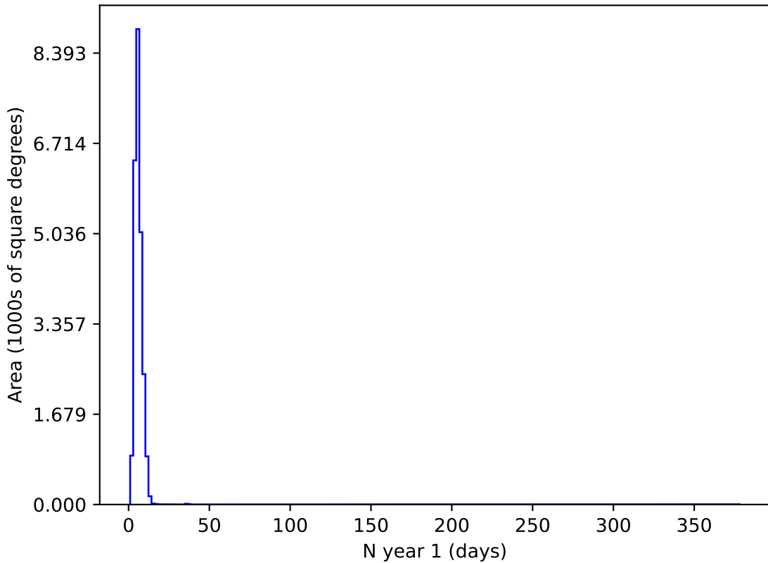
weather_cloudso8v3.4_10yrs u and night < 365: N year 1
