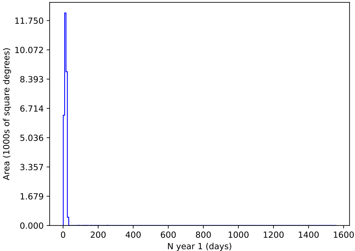
weather_cloudso8v3.4_10yrs r and night < 365: N year 1
