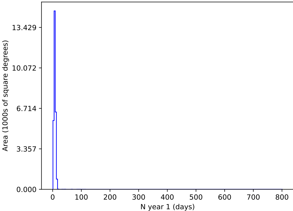
weather_cloudso8v3.4_10yrs g and night < 365: N year 1
