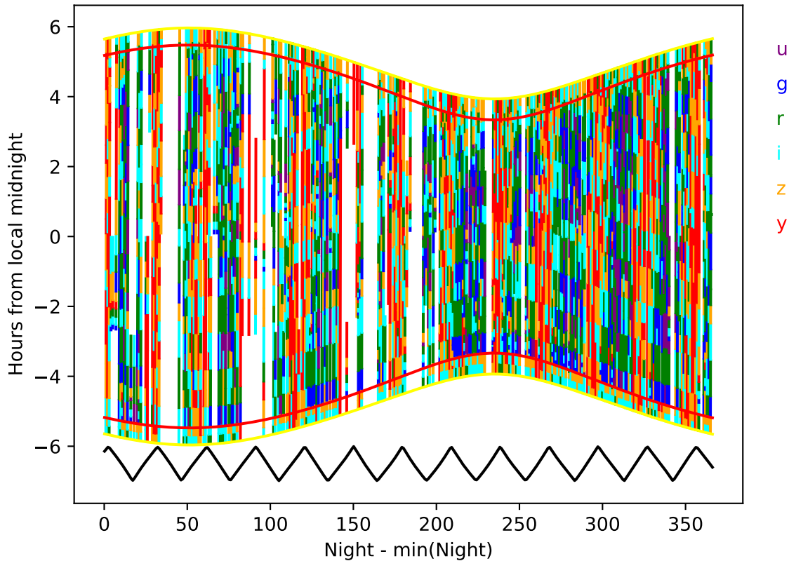
weather_cloudso8v3.4_10yrs year 9-10: Hourglass
