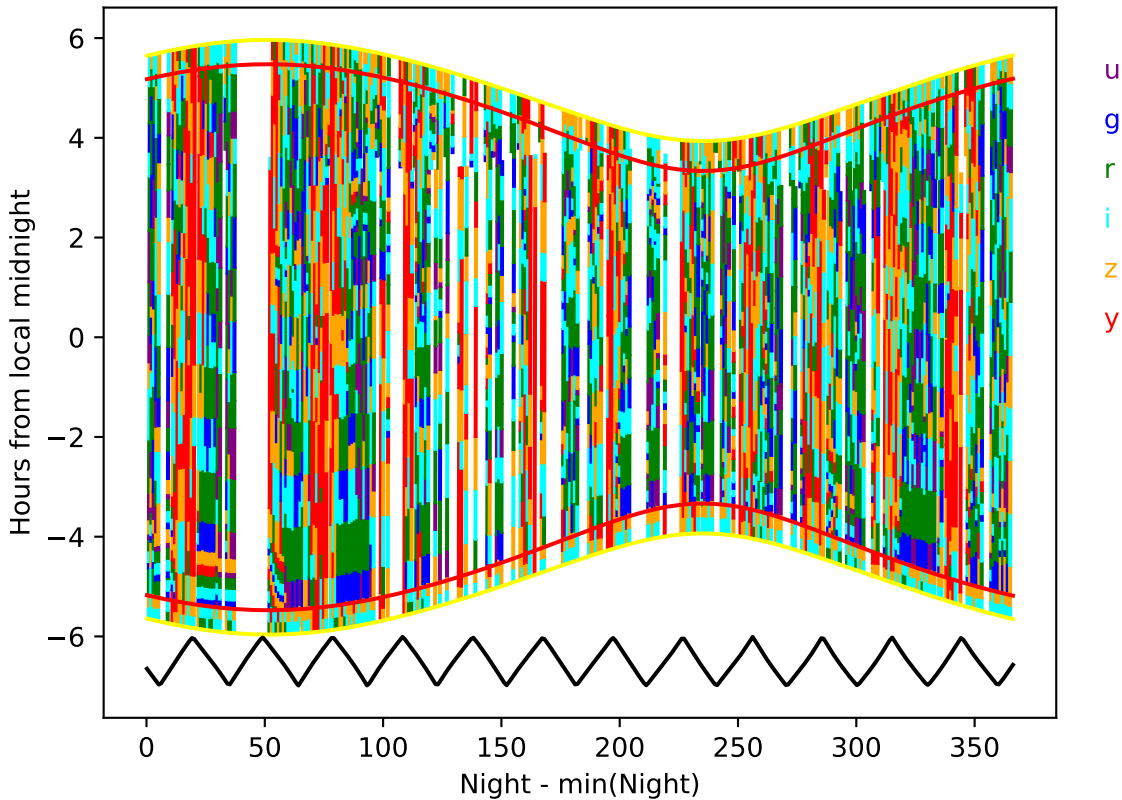
weather_cloudso8v3.4_10yrs year 2-3: Hourglass
