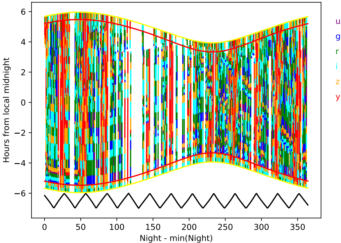
weather_cloudso8v3.4_10yrs year 1-2: Hourglass
