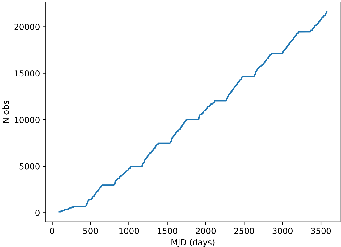
weather_cloudso8v3.4_10yrs note like DD:XMM_LSS%: Cumulative
