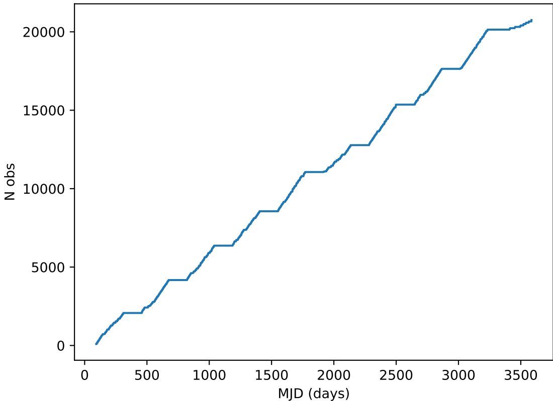
weather_cloudso8v3.4_10yrs note like DD:ECDFS%: Cumulative
