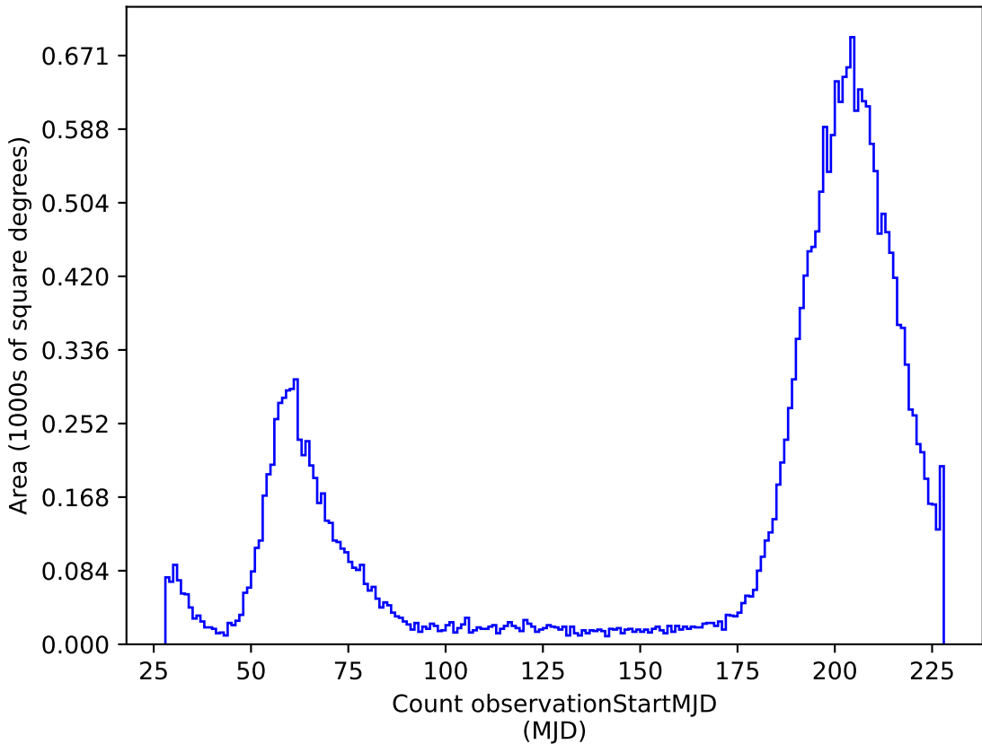
weather_cloudso8v3.4_10yrs i: Count observationStartMJD
