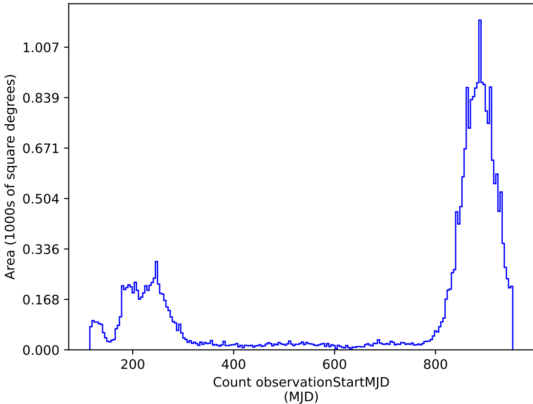
weather_cloudso8v3.4_10yrs : Count observationStartMJD
