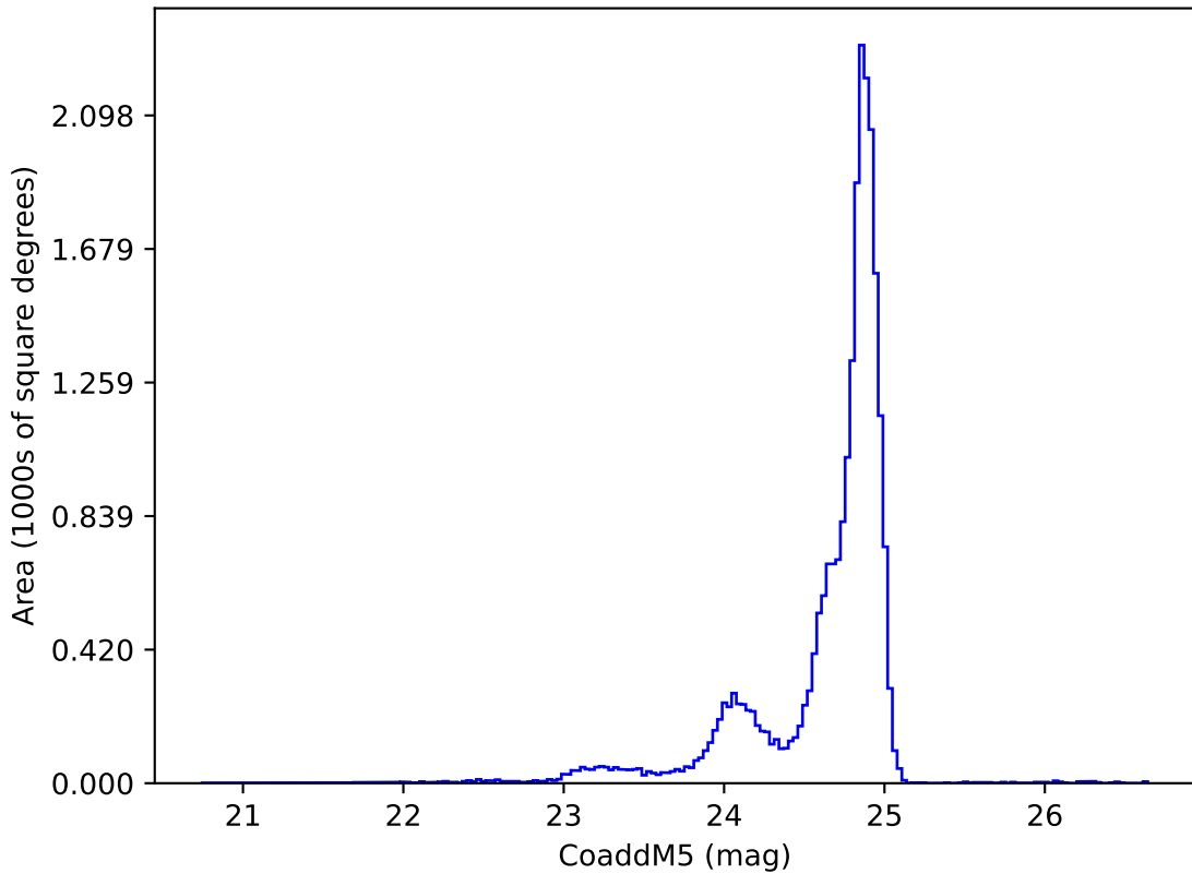
weather_cloudso8v3.4_10yrs y: CoaddM5
