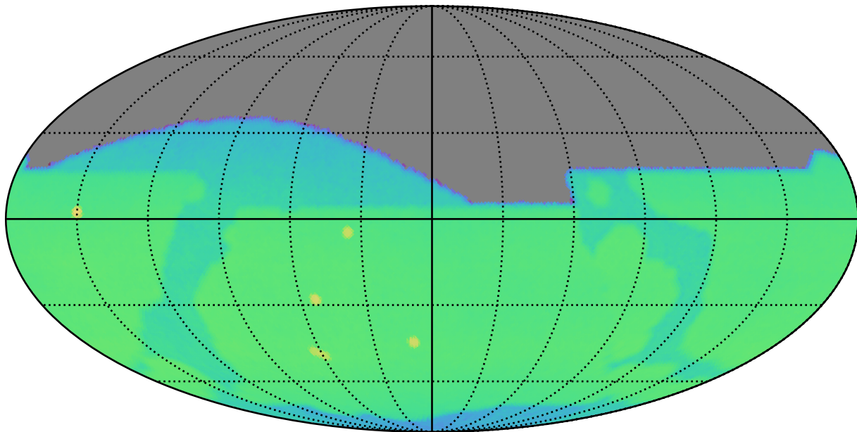
weather_cloudso8v3.4_10yrs r: CoaddM5
