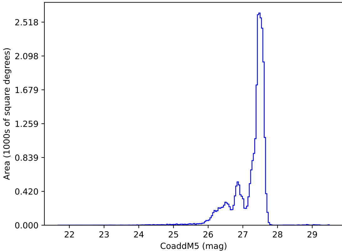
weather_cloudso8v3.4_10yrs : CoaddM5
