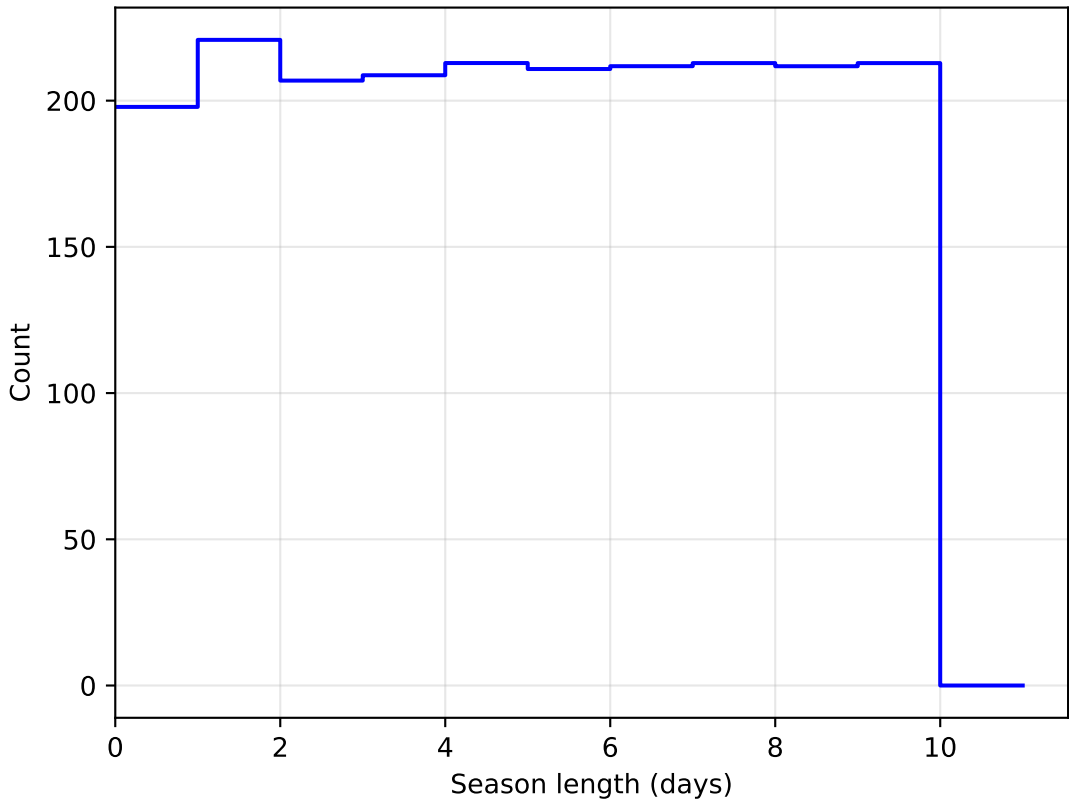
weather_cloudso8v3.4_10yrs DD:ELAISS1 all bands: SeasonLength
