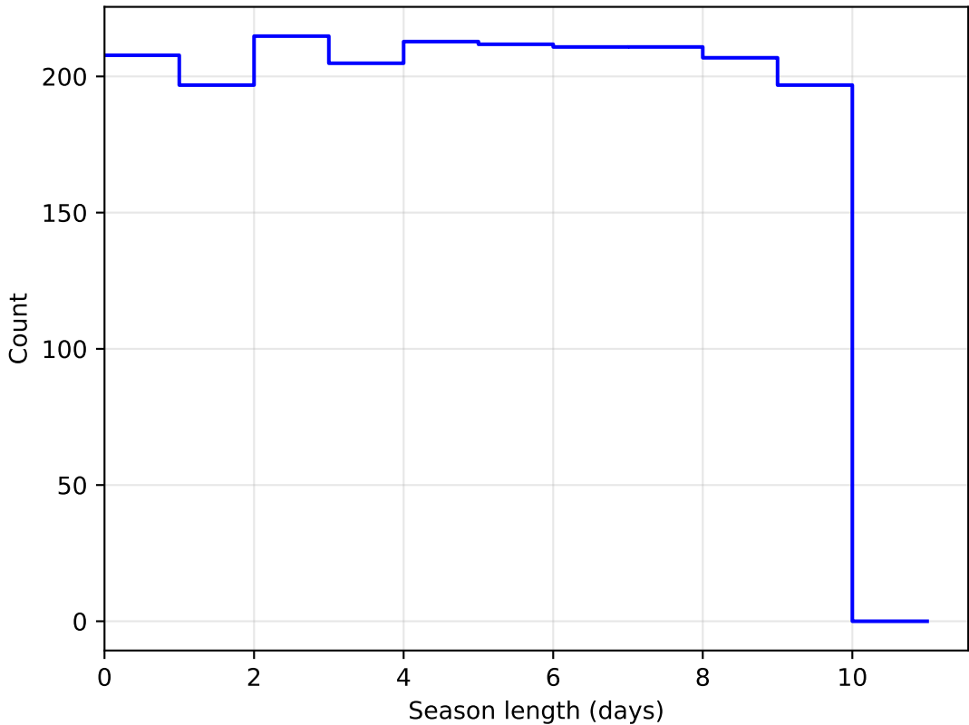
weather_cloudso8v3.4_10yrs DD:EDFS all bands: SeasonLength
