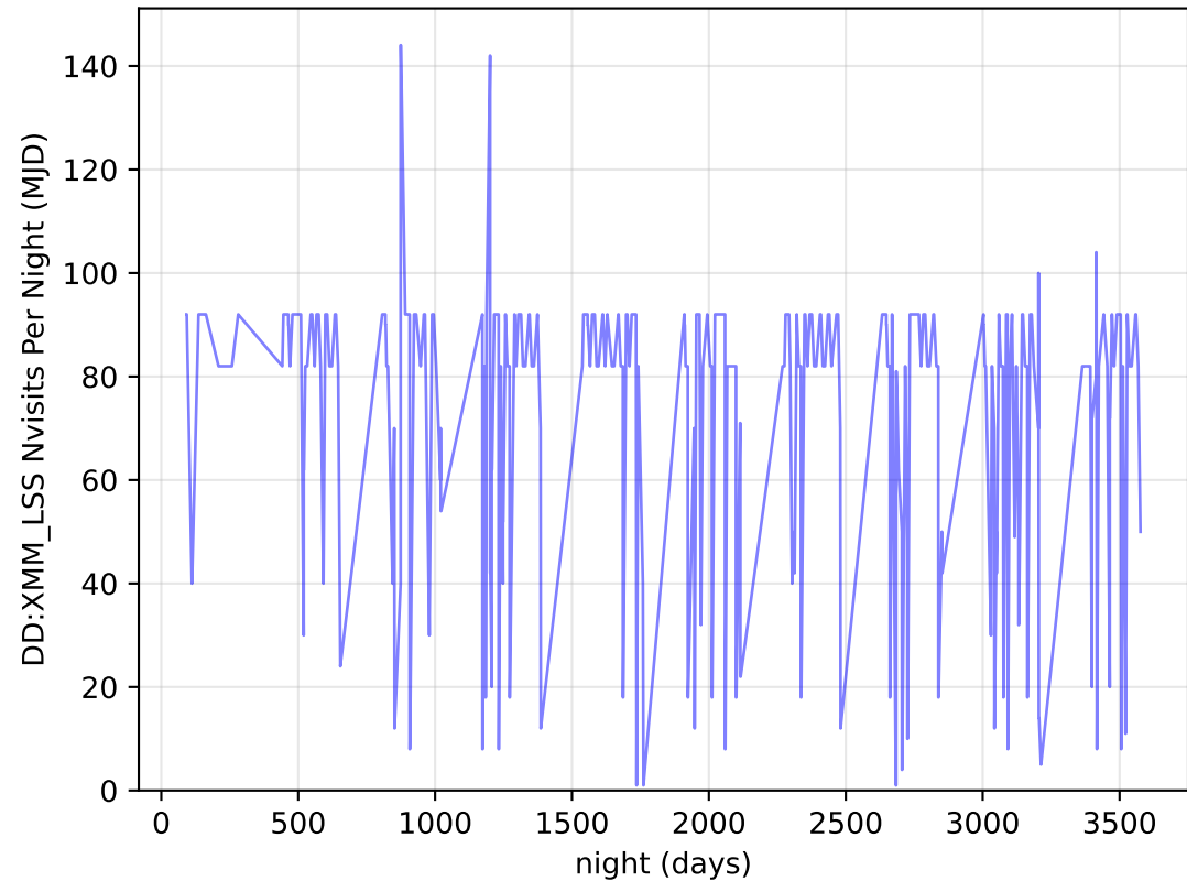
weather_cloudso8v3.4_10yrs all bands: DD:XMM_LSS Nvisits Per Night
