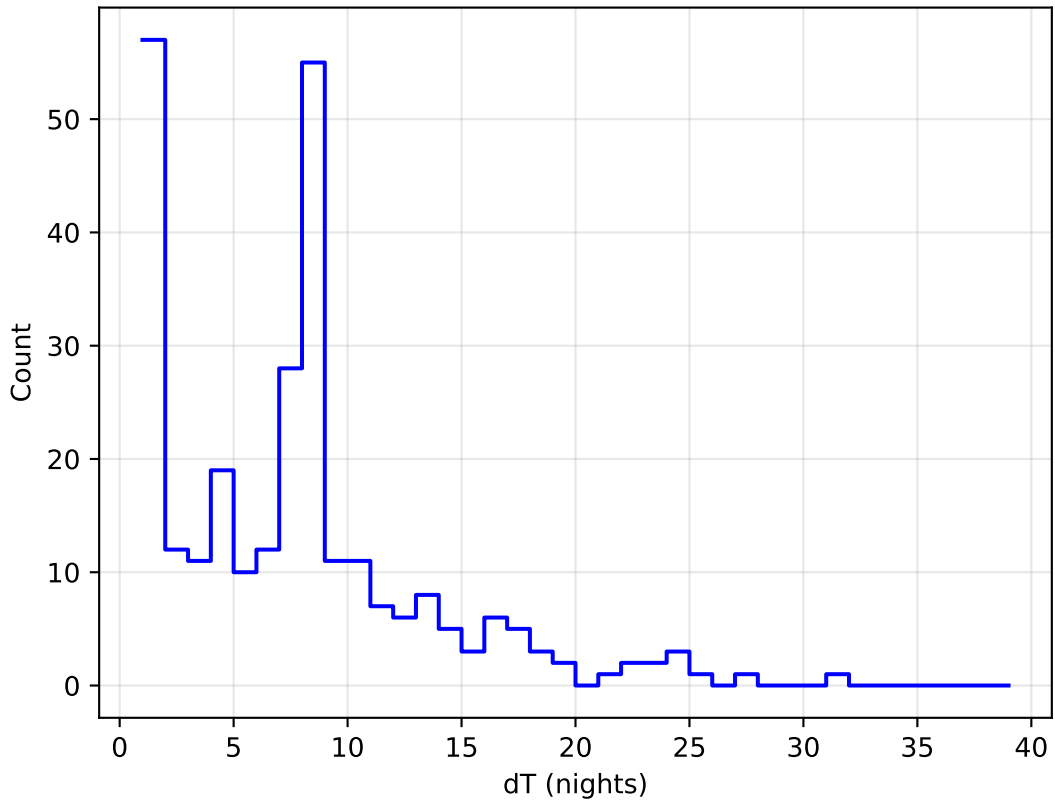
weather_cloudso8v3.4_10yrs all bands: DD:XMM_LSS Delta Nights Histogram
