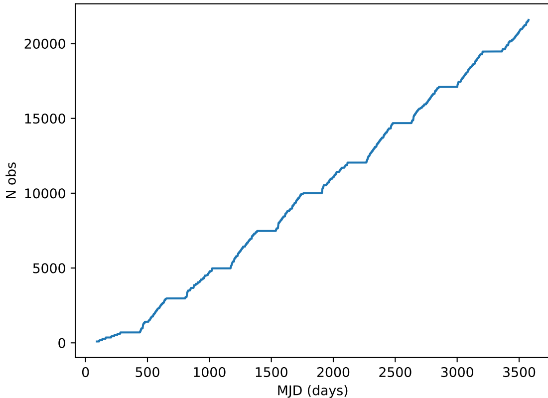
weather_cloudso8v3.4_10yrs all bands: DD:XMM_LSS Cumulative NVisits
