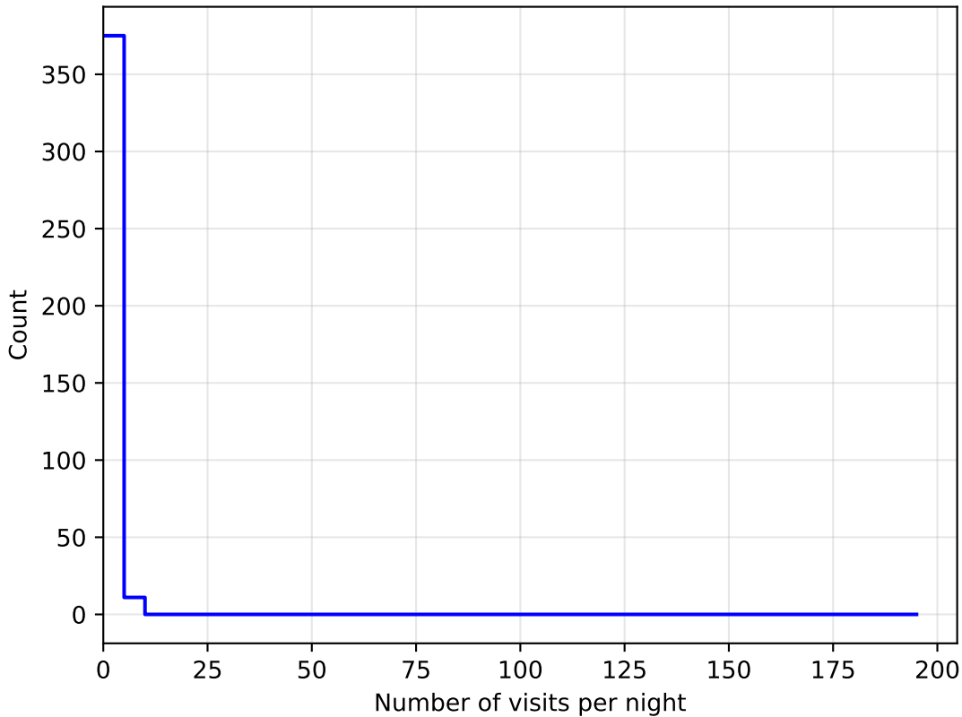
weather_cloudso8v3.4_10yrs all bands: DD:WFD NVisitsPerNight
