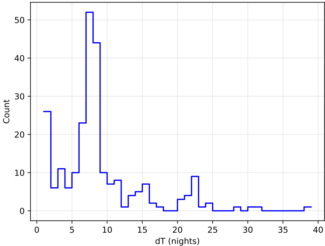
weather_cloudso8v3.4_10yrs all bands: DD:EDFS Delta Nights Histogram
