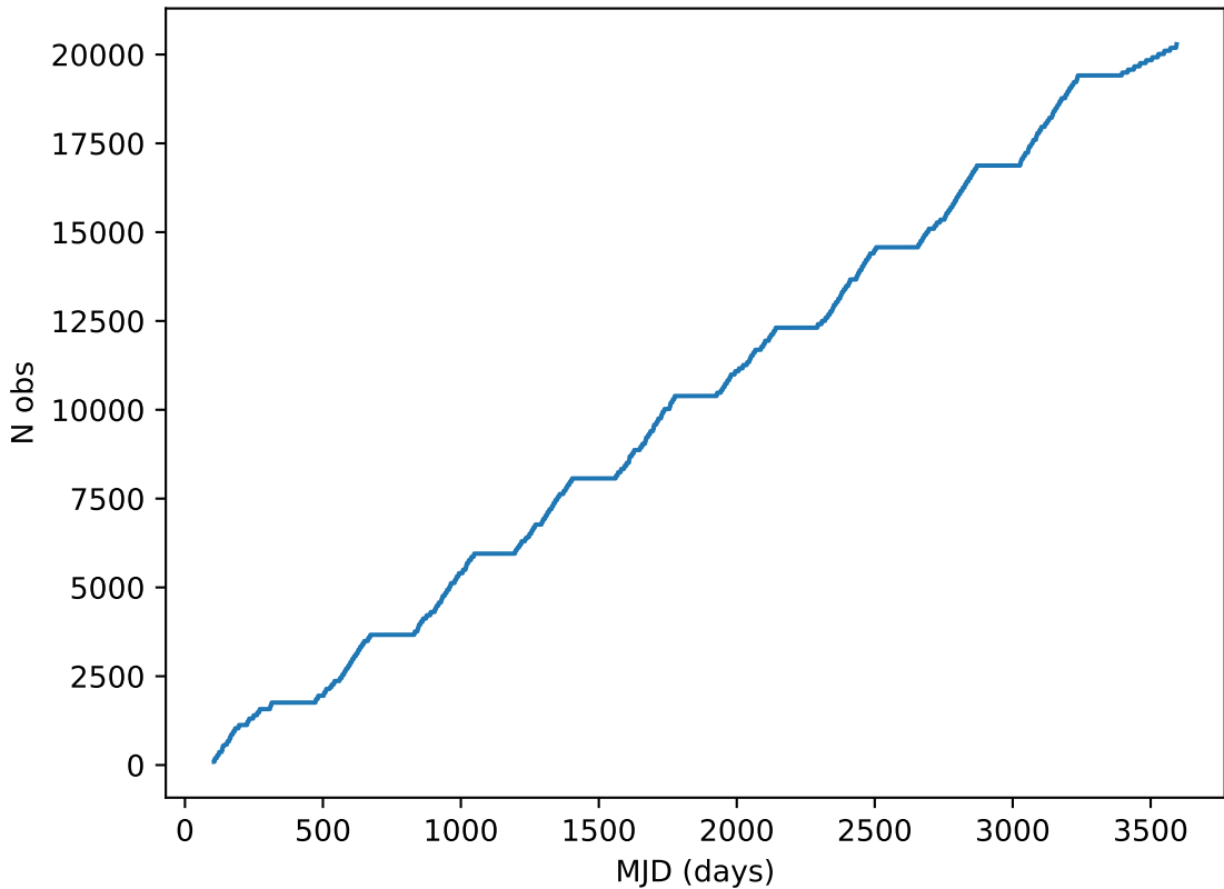
weather_cloudso8v3.4_10yrs all bands: DD:EDFS Cumulative NVisits
