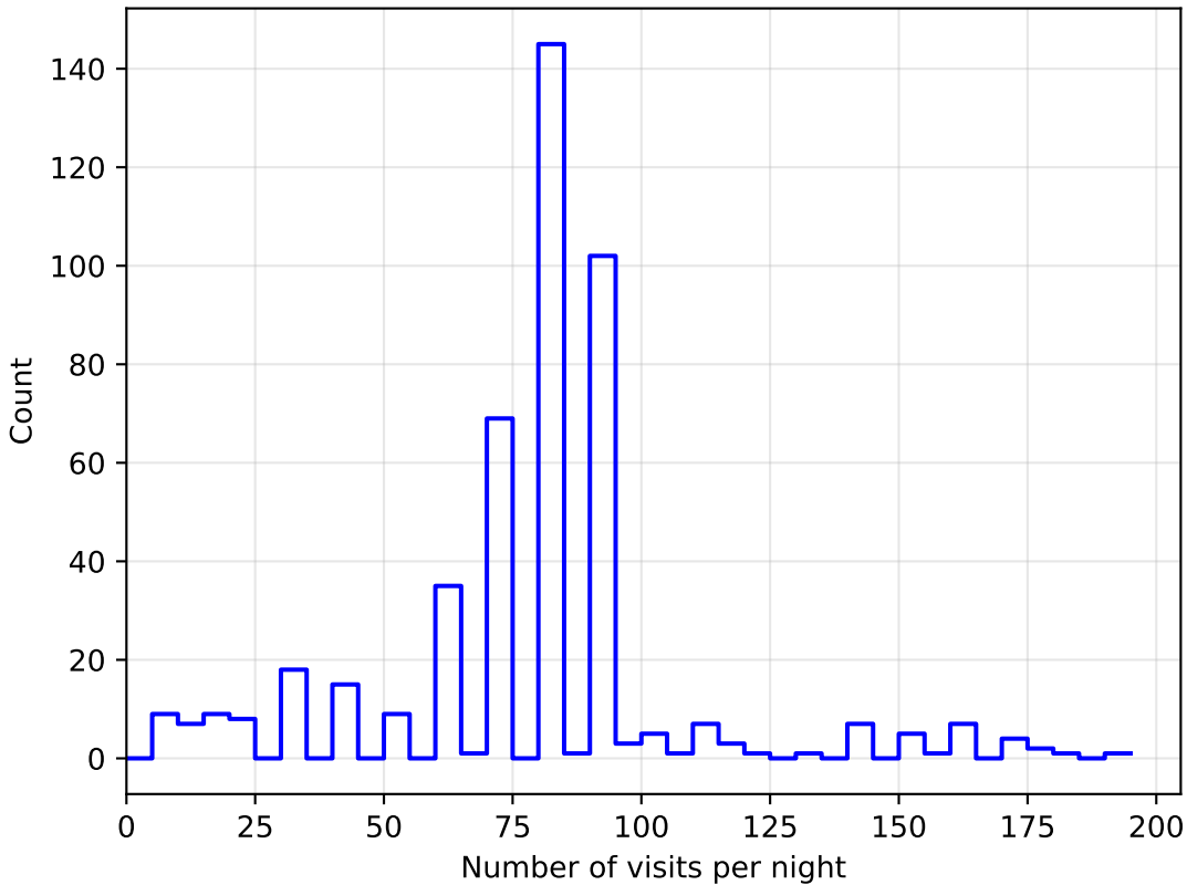
weather_cloudso8v3.4_10yrs all bands: DD:COSMOS NVisitsPerNight
