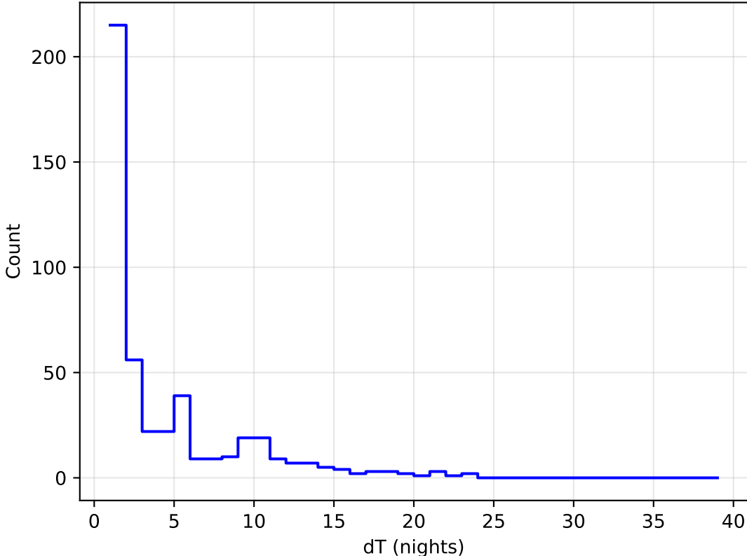
weather_cloudso8v3.4_10yrs all bands: DD:COSMOS Delta Nights Histogram
