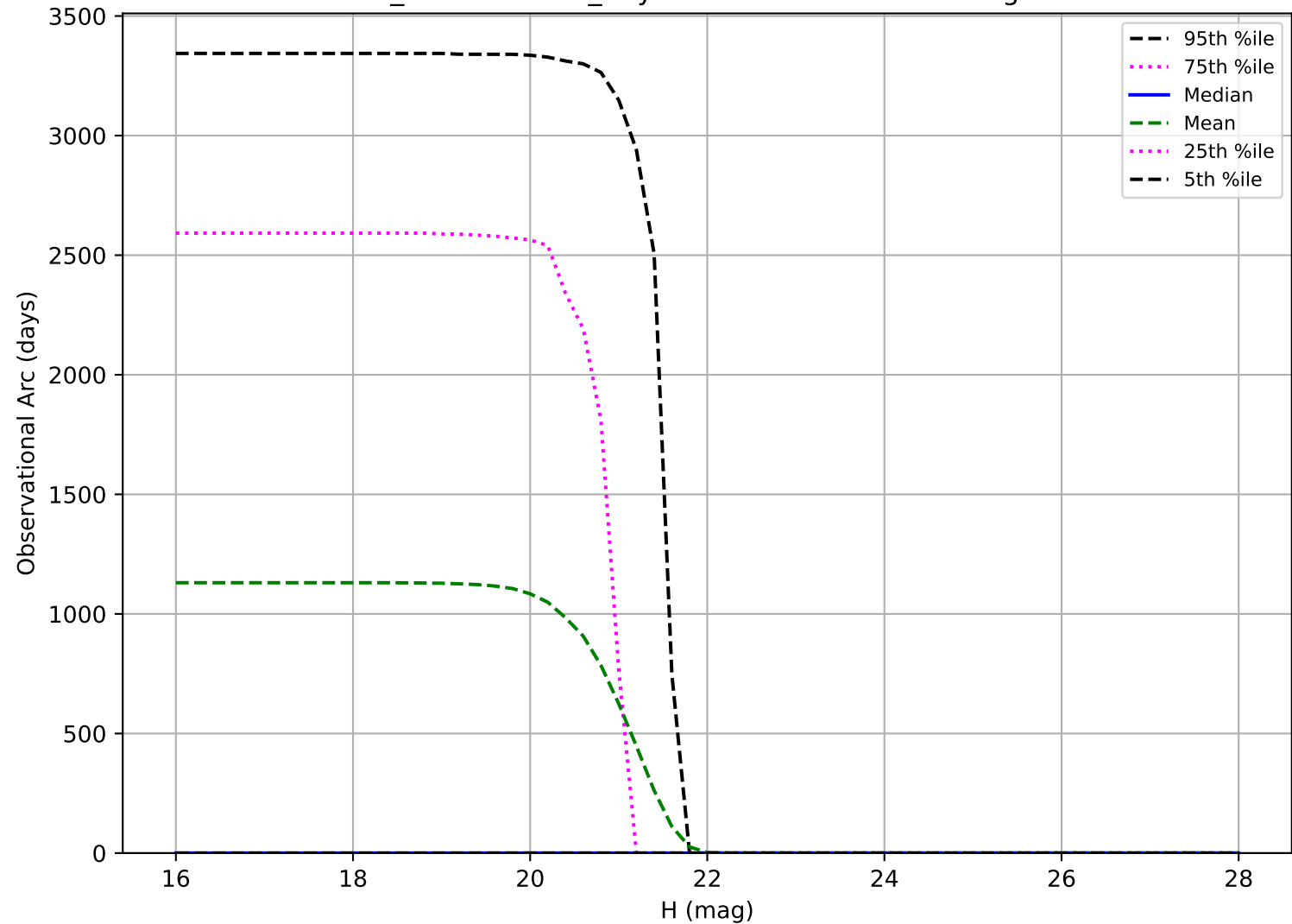
weather_cloudso6v3.4_10yrs: Observational Arc Length Vatira
