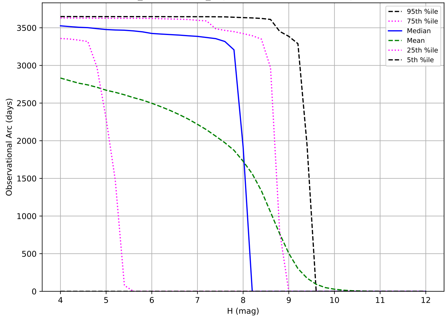
weather_cloudso6v3.4_10yrs: Observational Arc Length TNO
