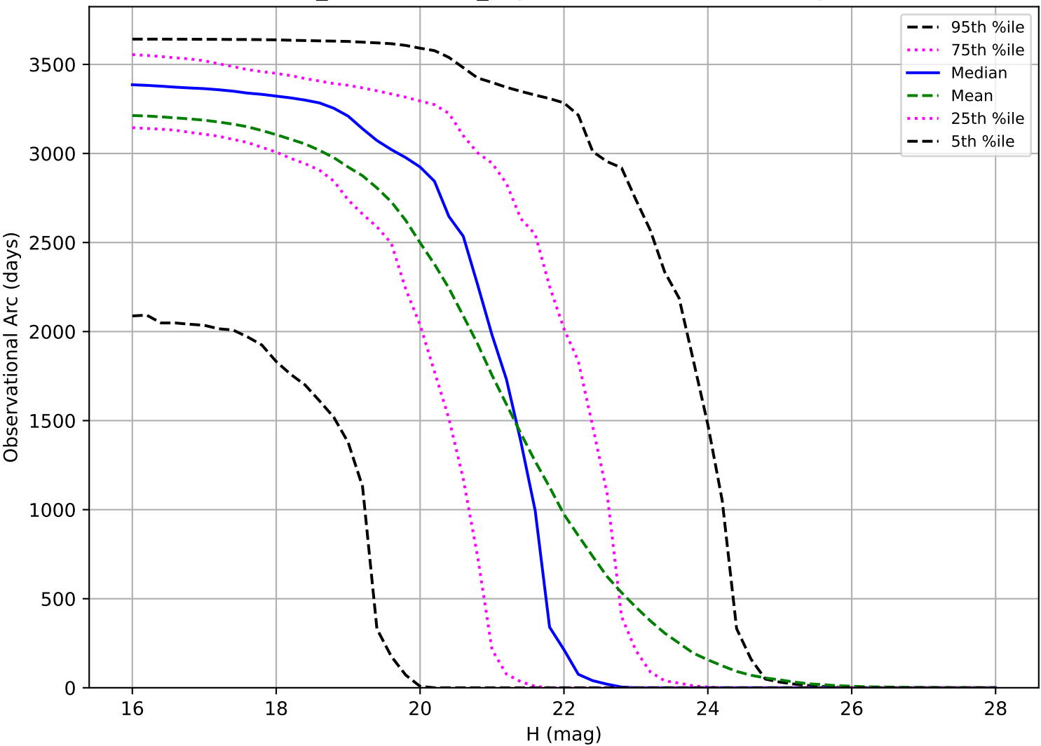
weather_cloudso6v3.4_10yrs: Observational Arc Length PHA
