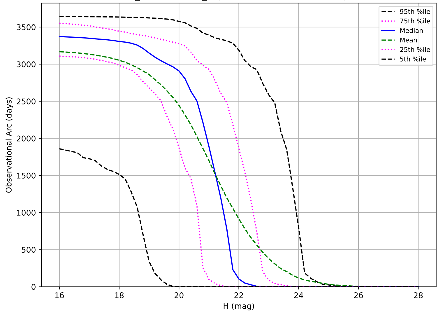
weather_cloudso6v3.4_10yrs: Observational Arc Length NEO
