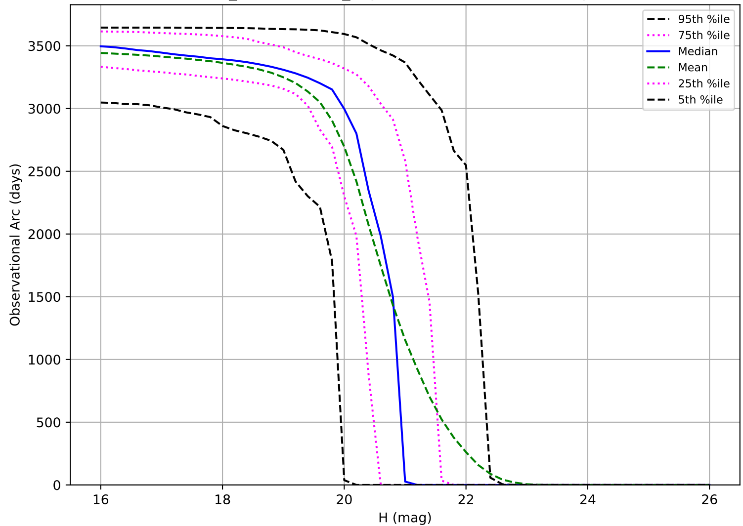
weather_cloudso6v3.4_10yrs: Observational Arc Length MBA
