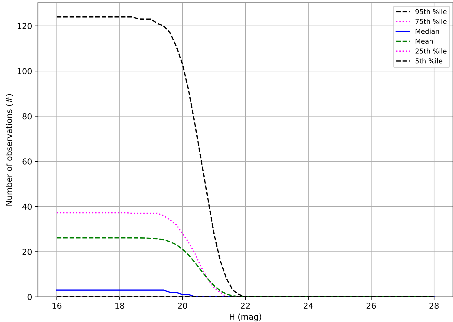
weather_cloudso6v3.4_10yrs: Number of observations Vatira
