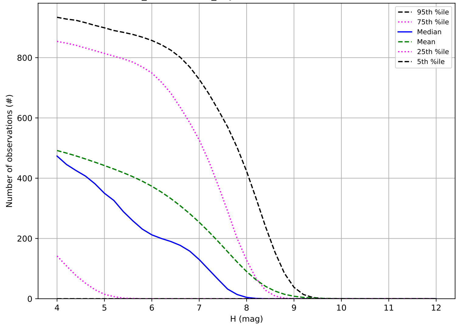
weather_cloudso6v3.4_10yrs: Number of observations TNO
