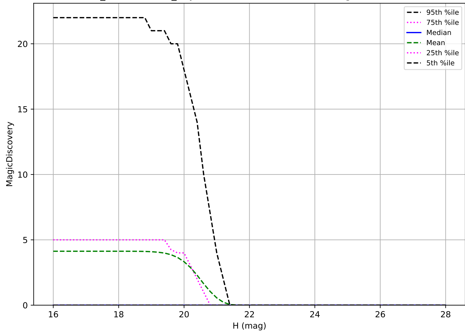
weather_cloudso6v3.4_10yrs: Vatira 6 detections in 60 nights detection loss
