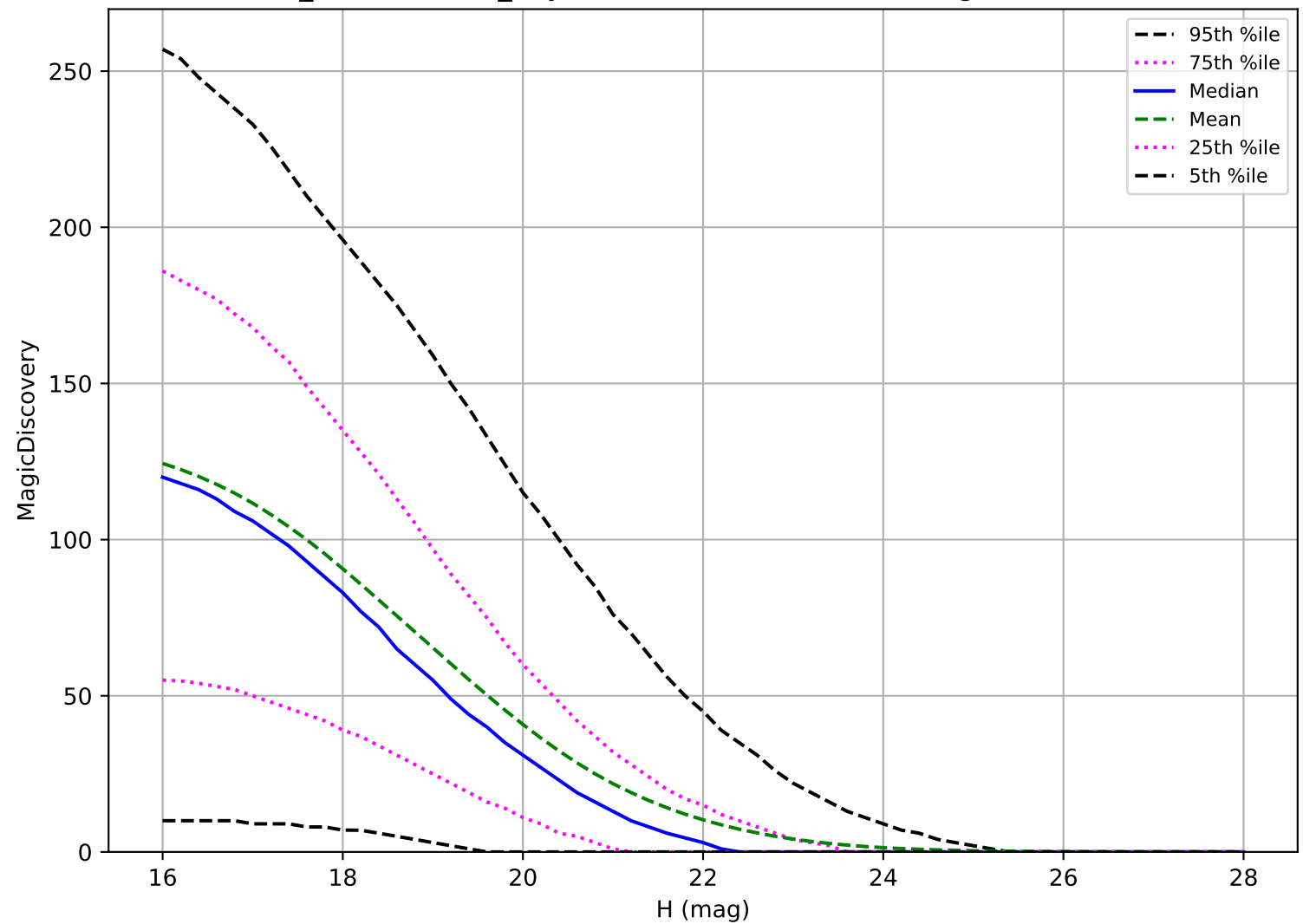
weather_cloudso6v3.4_10yrs: PHA 6 detections in 60 nights detection loss
