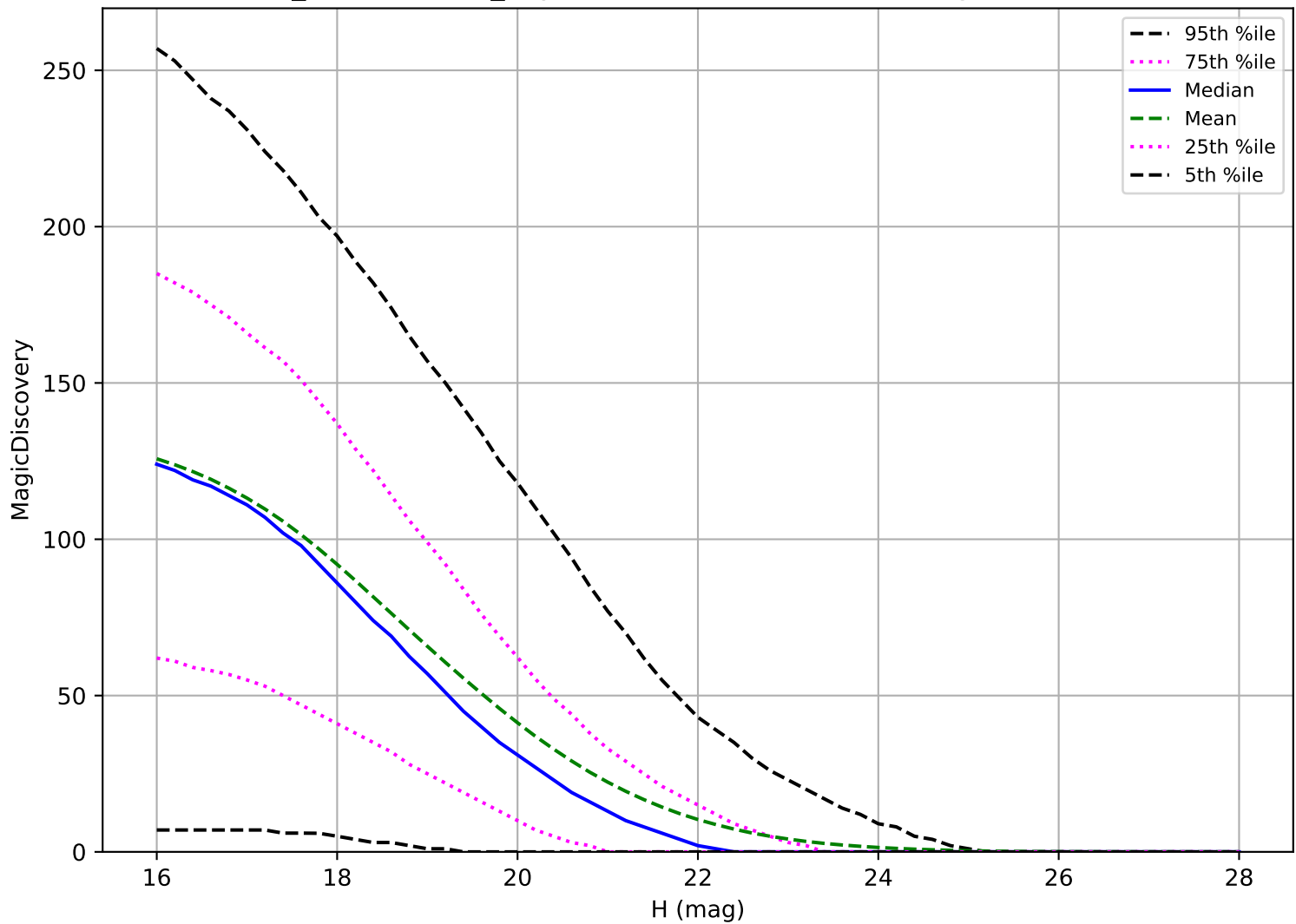
weather_cloudso6v3.4_10yrs: NEO 6 detections in 60 nights detection loss
