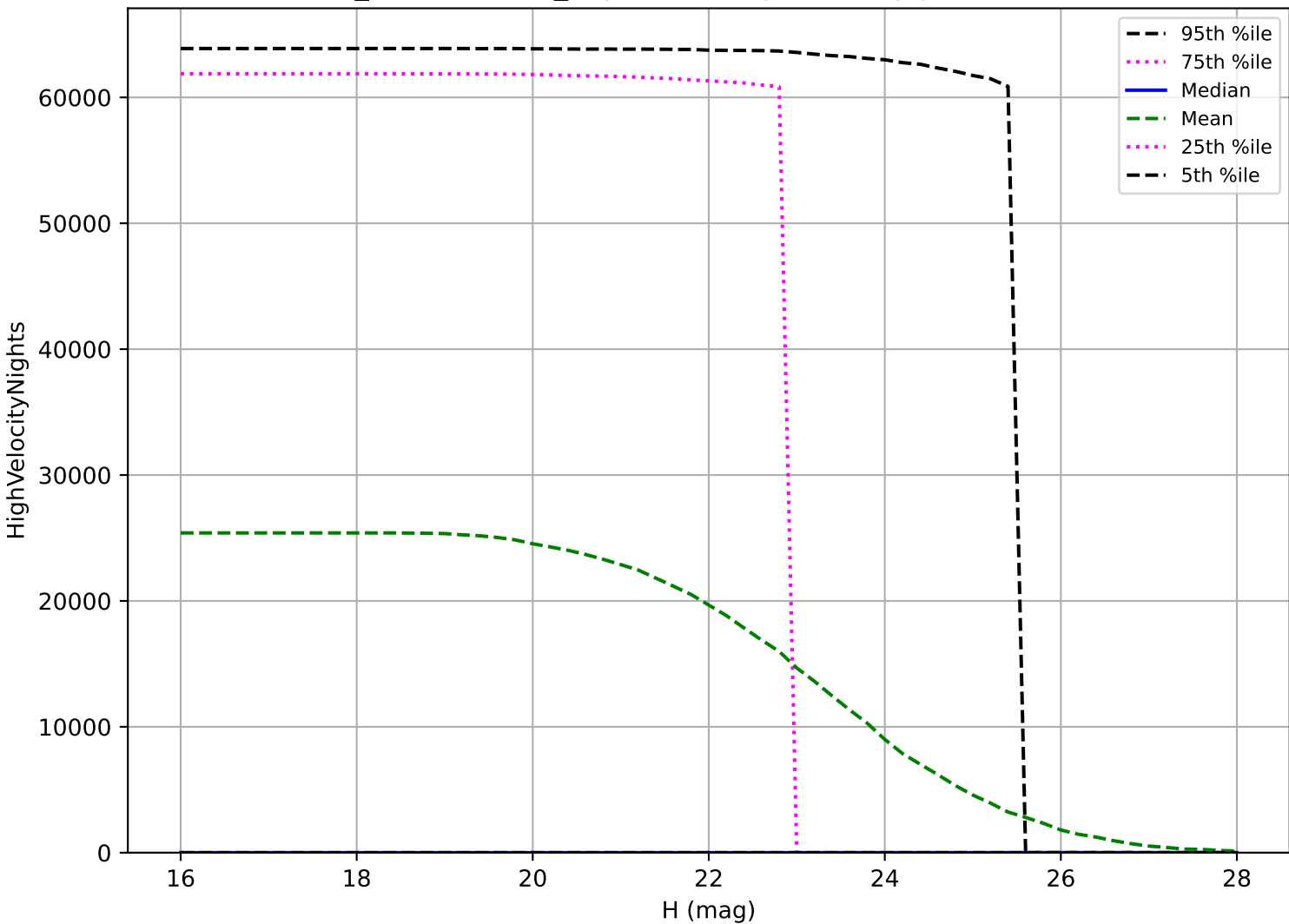
weather_cloudso6v3.4_10yrs: PHA High velocity pair detection loss
