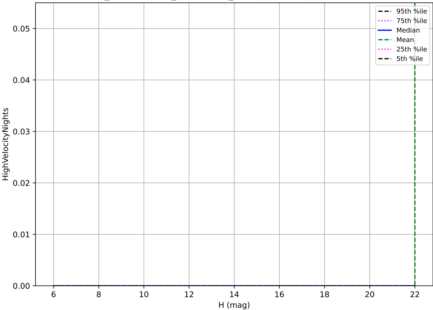
weather_cloudso6v3.4_10yrs: OCC_r20 High velocity pair detection loss
