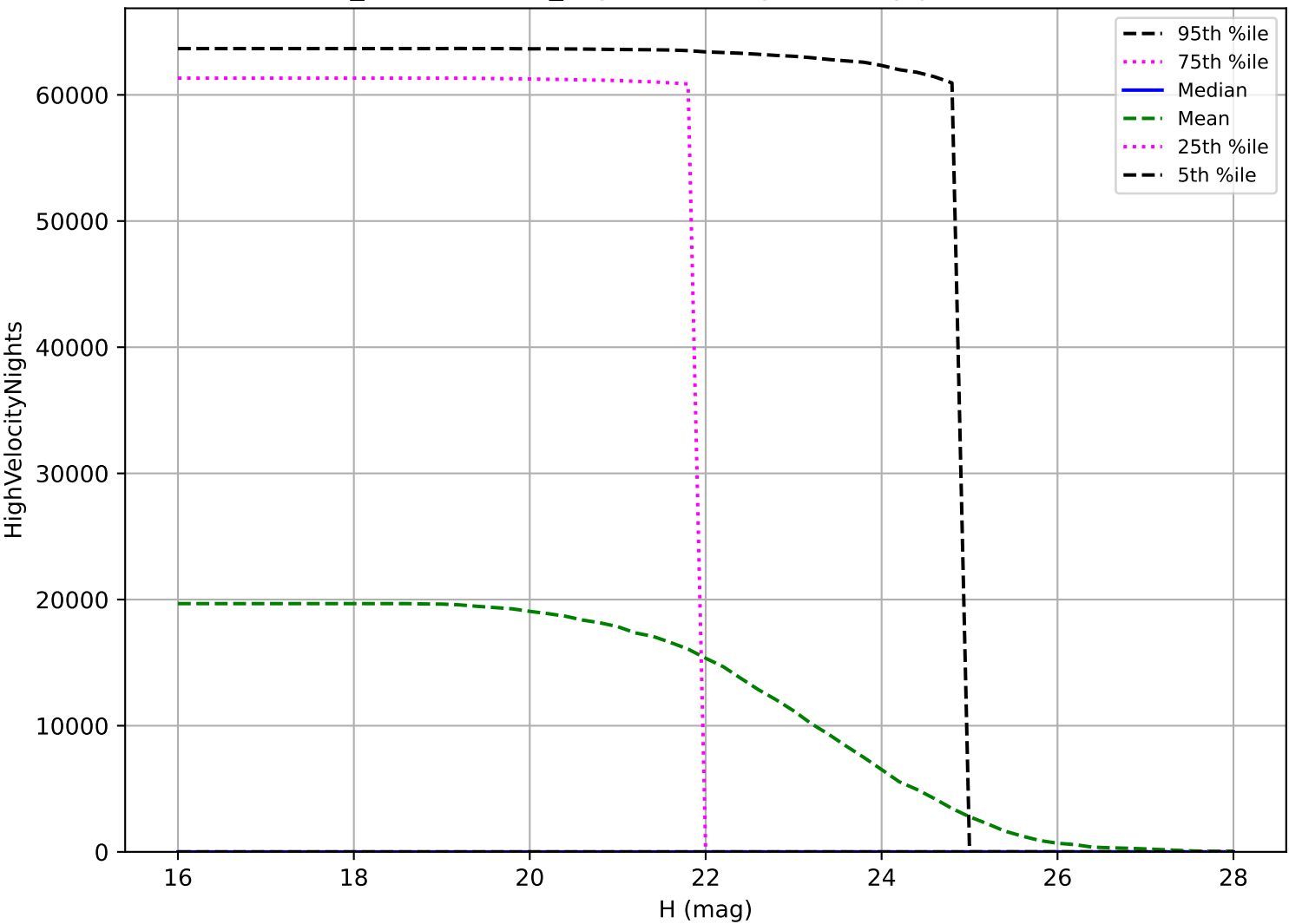
weather_cloudso6v3.4_10yrs: NEO High velocity pair detection loss
