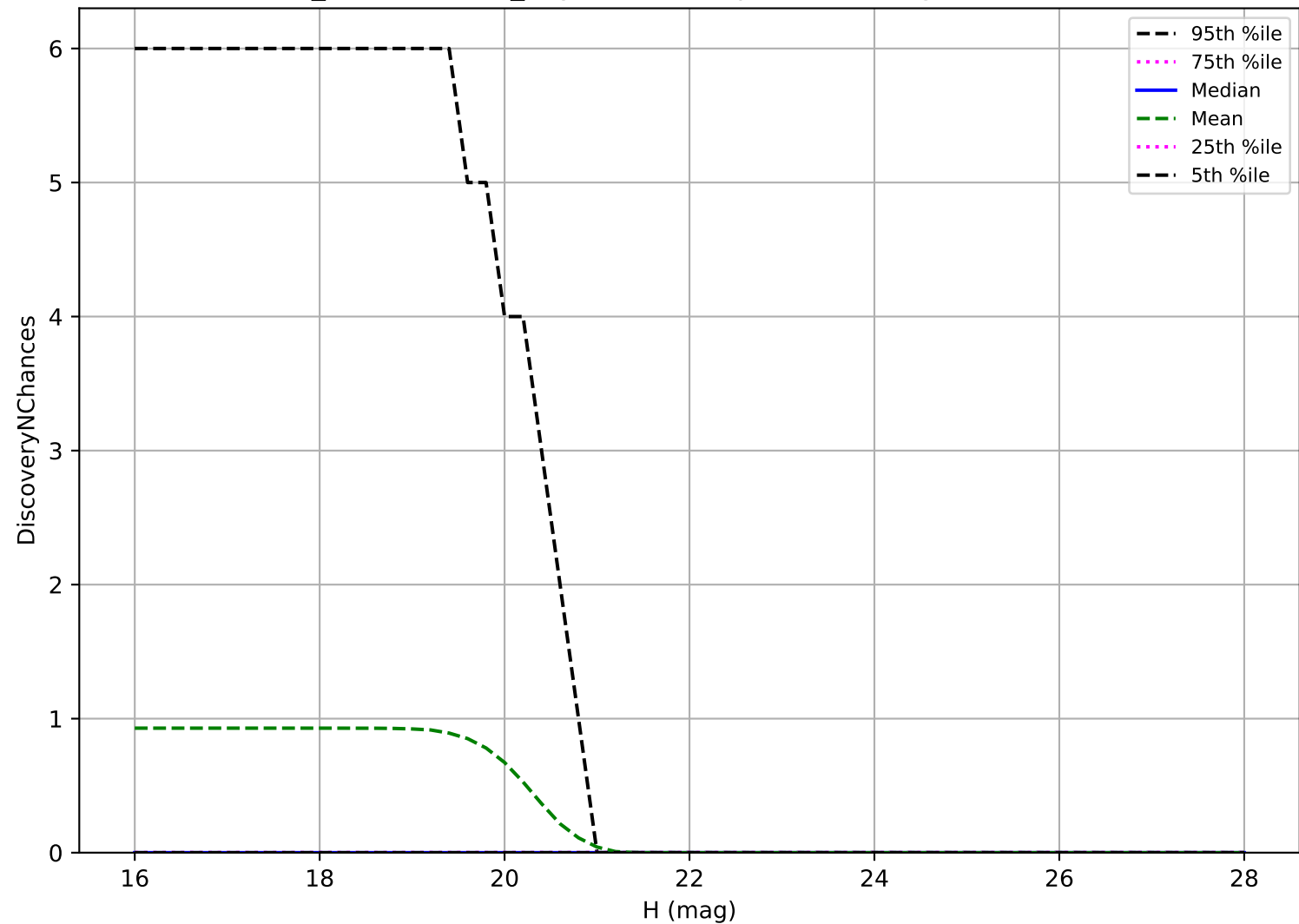
weather_cloudso6v3.4_10yrs: Vatira 3 pairs in 15 nights detection loss
