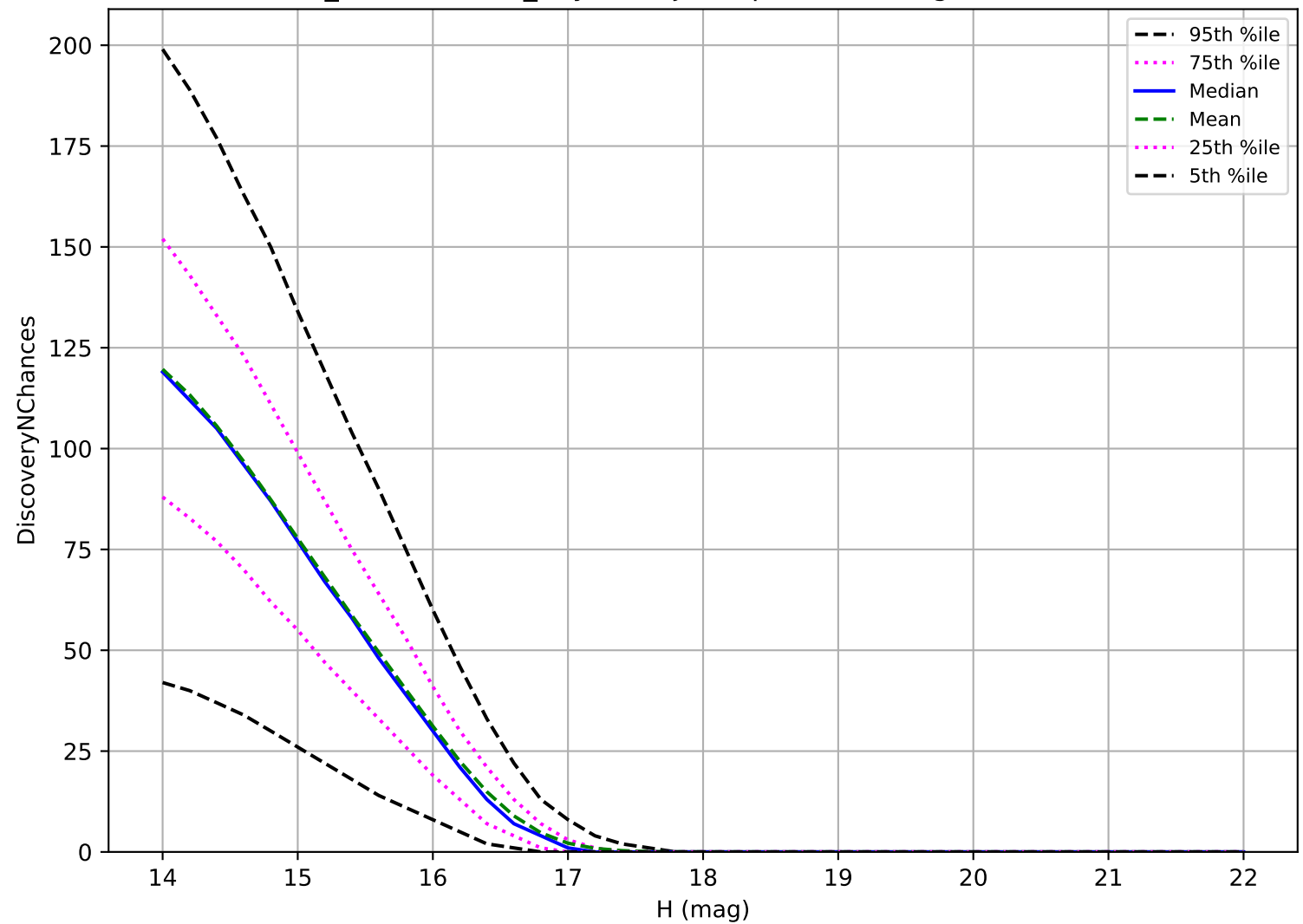
weather_cloudso6v3.4_10yrs: Trojan 3 pairs in 15 nights detection loss
