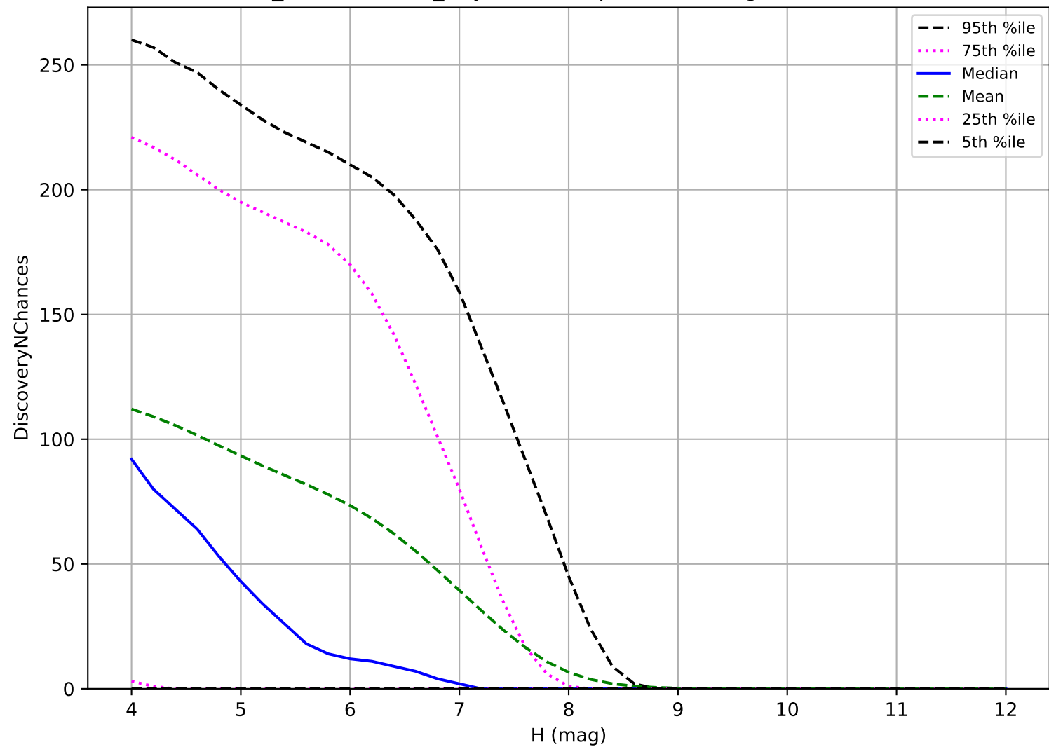
weather_cloudso6v3.4_10yrs: TNO 3 pairs in 15 nights detection loss
