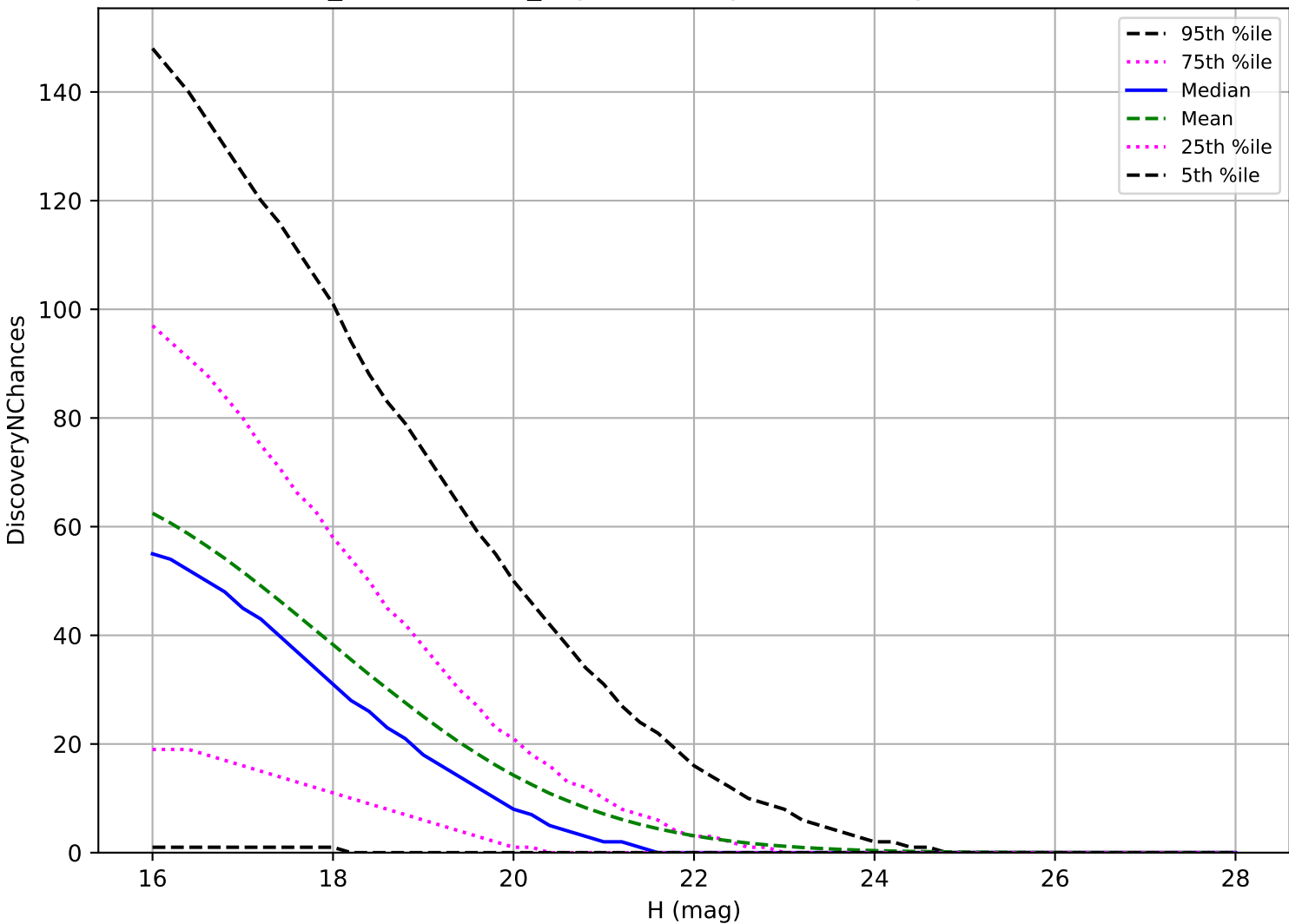
weather_cloudso6v3.4_10yrs: PHA 3 pairs in 15 nights detection loss
