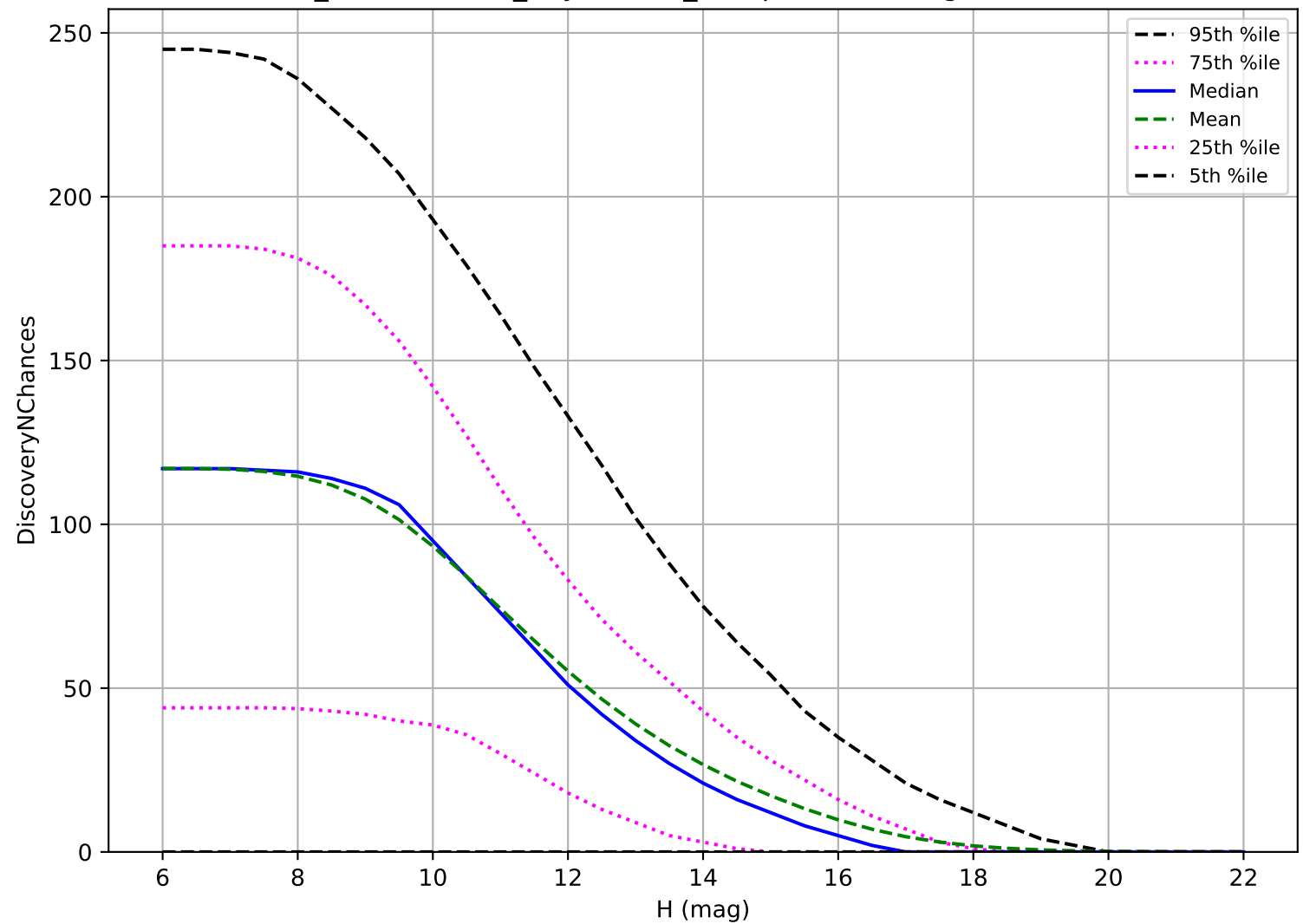
weather_cloudso6v3.4_10yrs: OCC_r5 3 pairs in 15 nights detection loss
