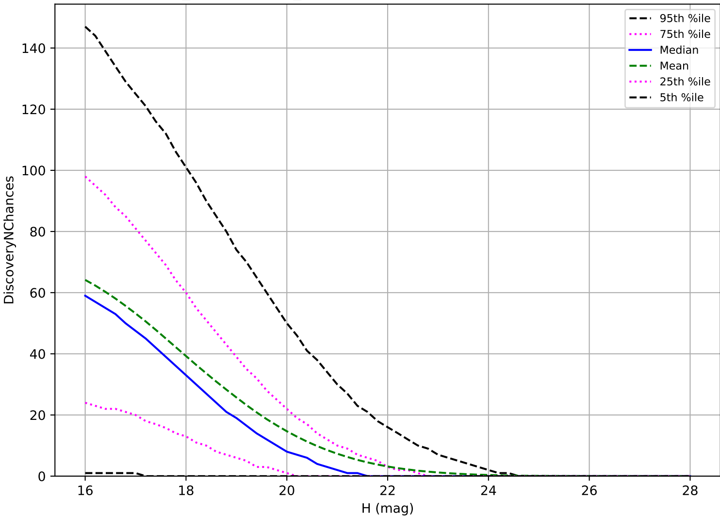
weather_cloudso6v3.4_10yrs: NEO 3 pairs in 15 nights detection loss
