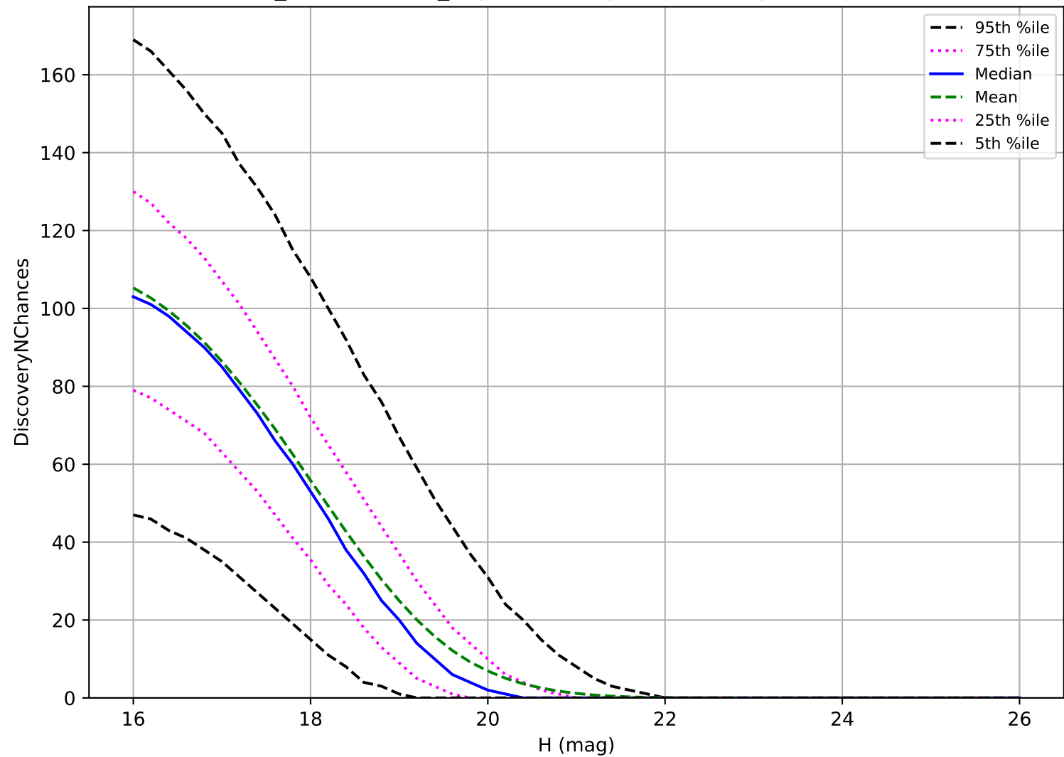
weather_cloudso6v3.4_10yrs: MBA 3 pairs in 15 nights detection loss
