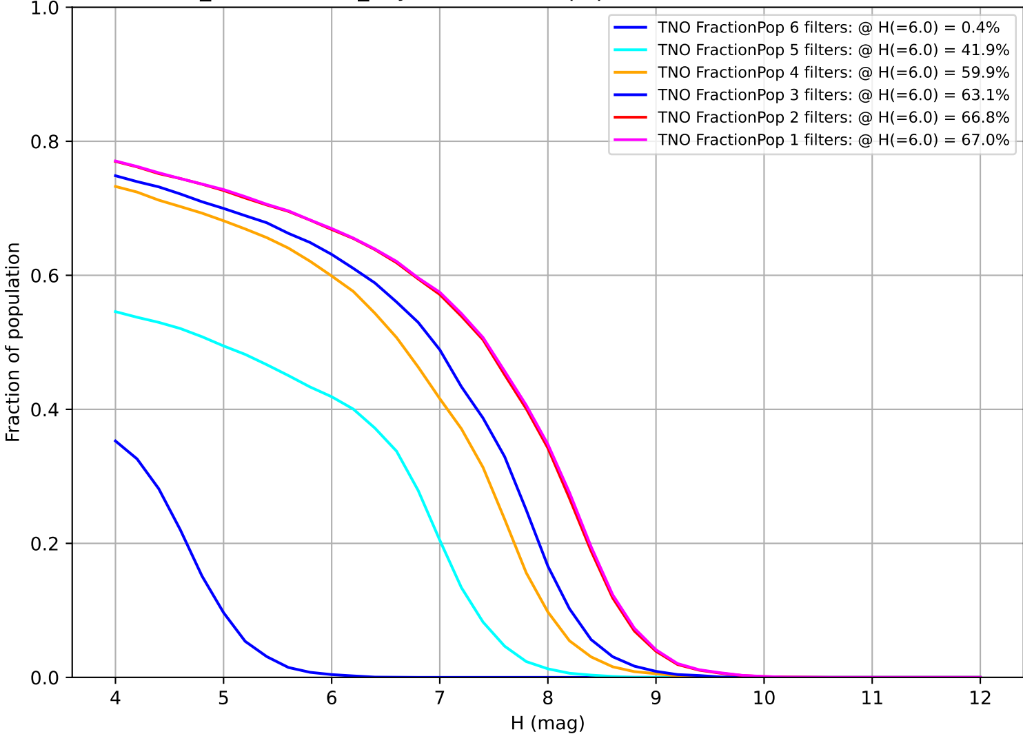
weather_cloudso6v3.4_10yrs: Fraction of population with colors in X filters TNO
