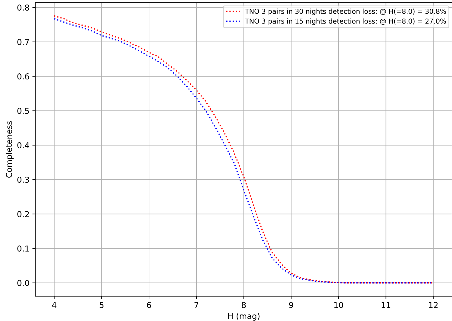
weather_cloudso6v3.4_10yrs: DifferentialCompleteness
