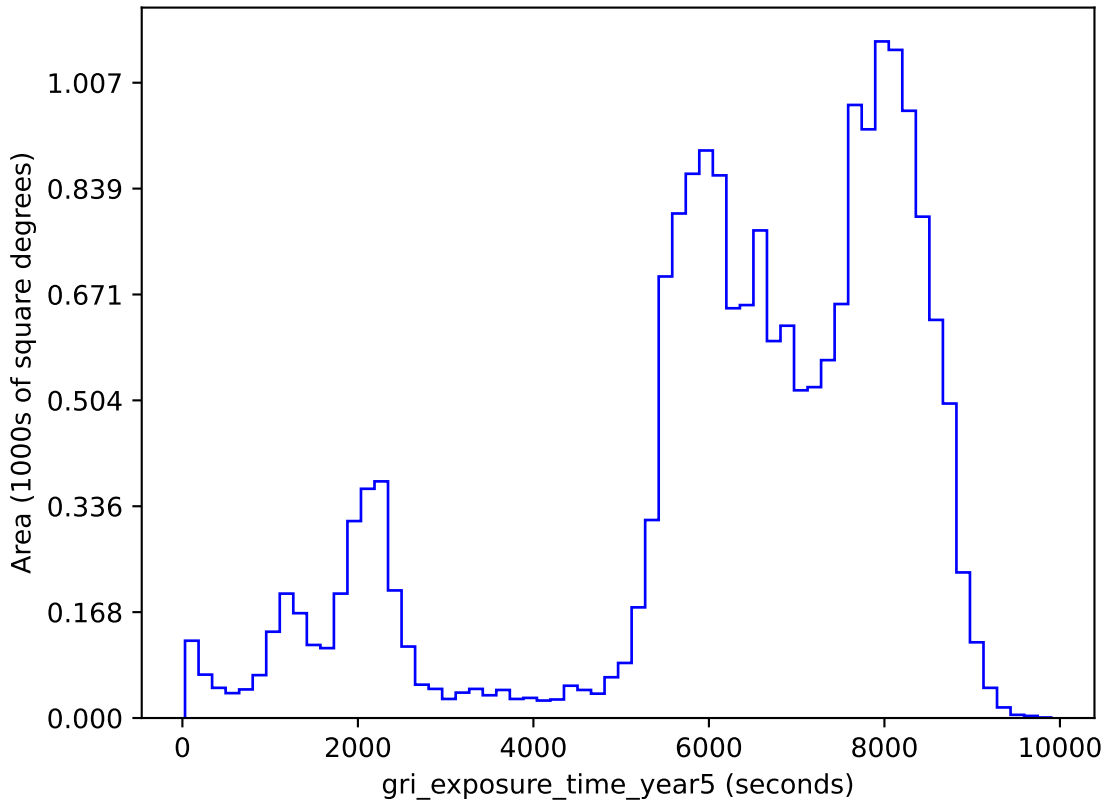
weather_cloudso6v3.4_10yrs gri band non-DD: gri_exposure_time_year5
