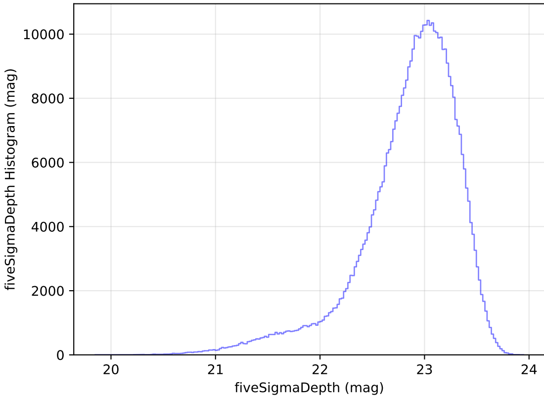
weather_cloudso6v3.4_10yrs z: fiveSigmaDepth Histogram
