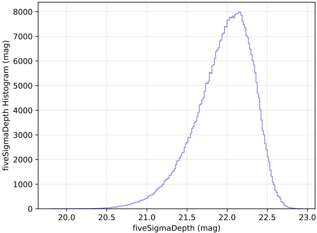
weather_cloudso6v3.4_10yrs y: fiveSigmaDepth Histogram
